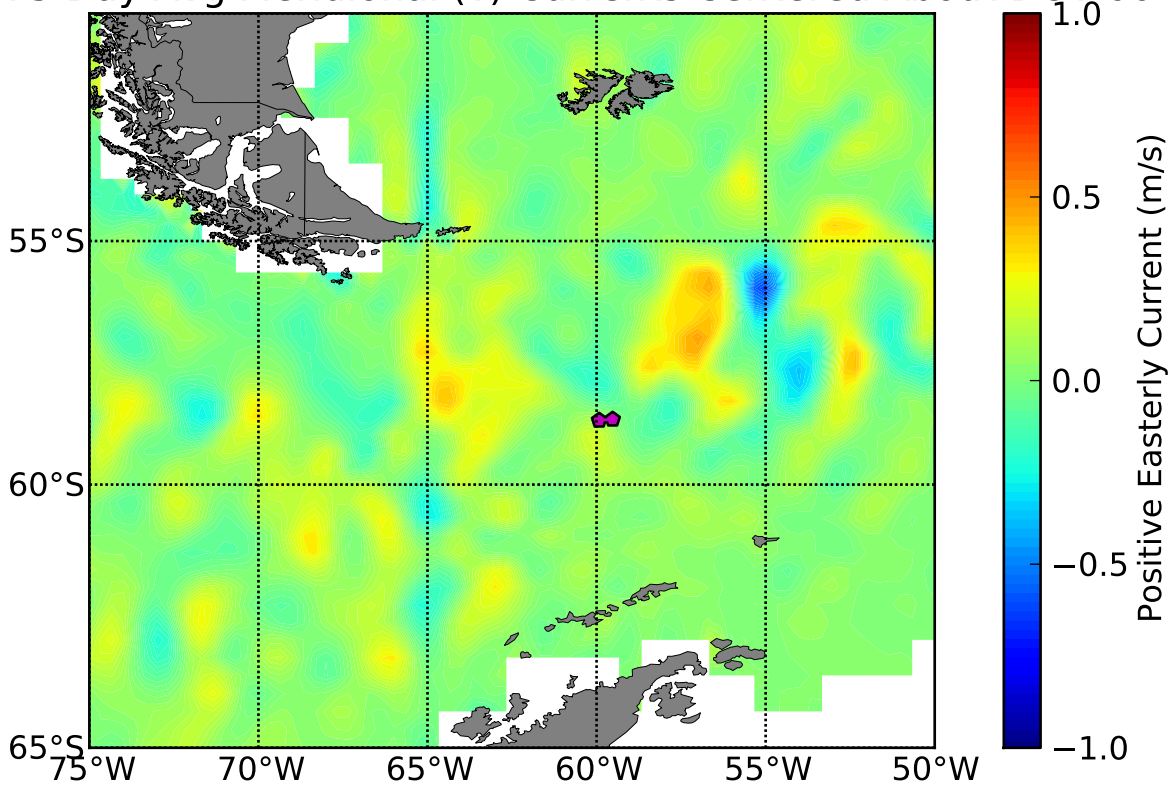
OSCAR 5 Day Avg Meridional (v) Currents Centered About DOY 66
