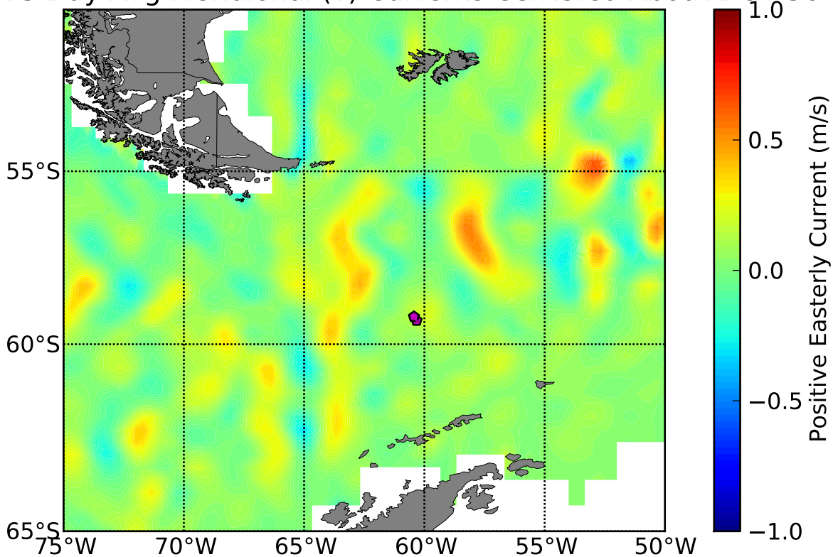
OSCAR 5 Day Avg Meridional (v) Currents Centered About DOY 56
