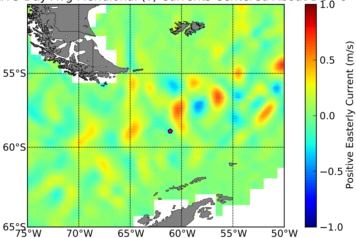
OSCAR 5 Day Avg Meridional (v) Currents Centered About DOY 6
