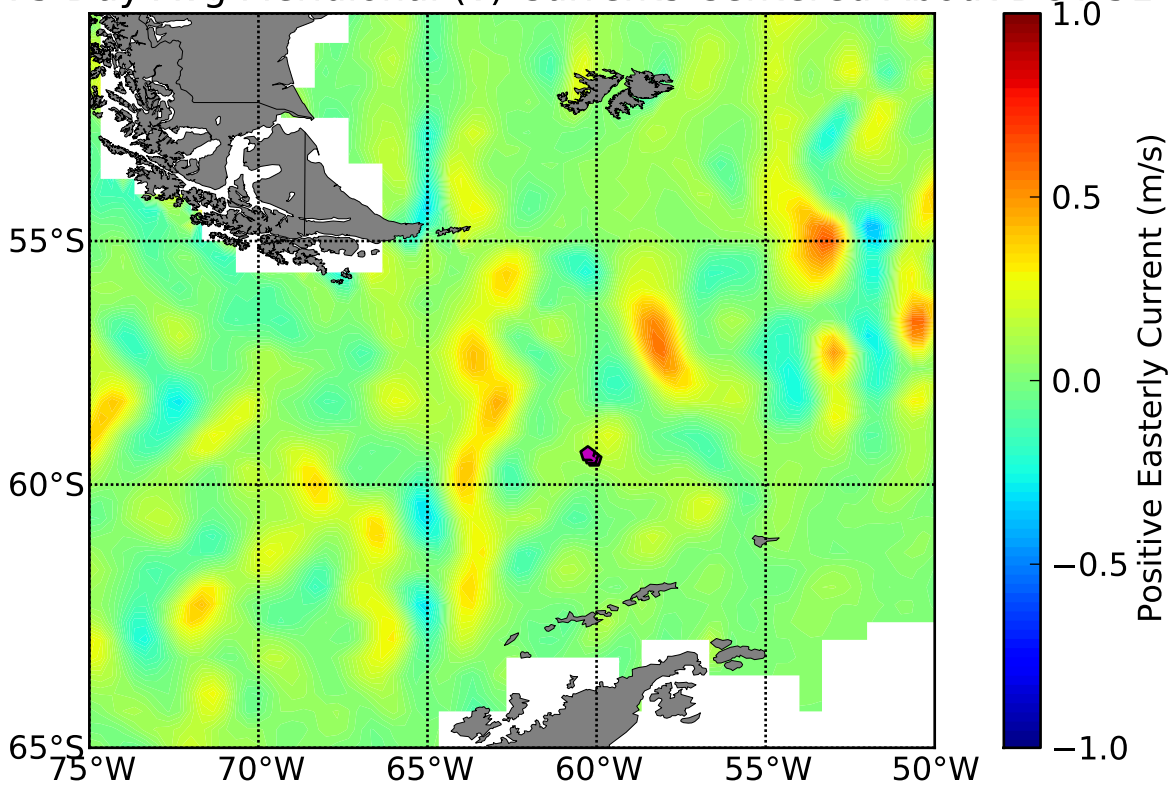
OSCAR 5 Day Avg Meridional (v) Currents Centered About DOY 51
