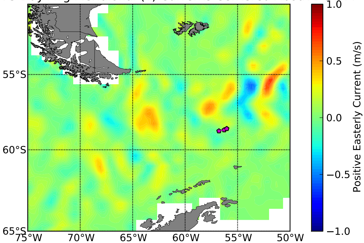
OSCAR 5 Day Avg Meridional (v) Currents Centered About DOY 77
