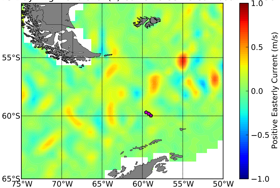
OSCAR 5 Day Avg Meridional (v) Currents Centered About DOY_36
