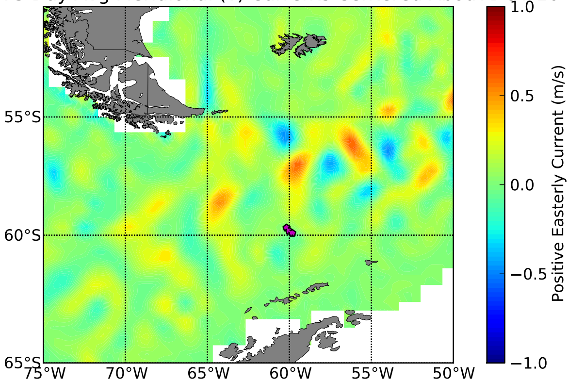
OSCAR 5 Day Avg Meridional (v) Currents Centered About DOY 16
