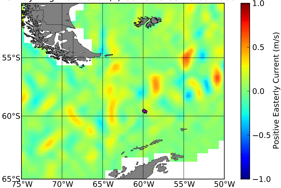
OSCAR 5 Day Avg Meridional (v) Currents Centered About DOY 41
