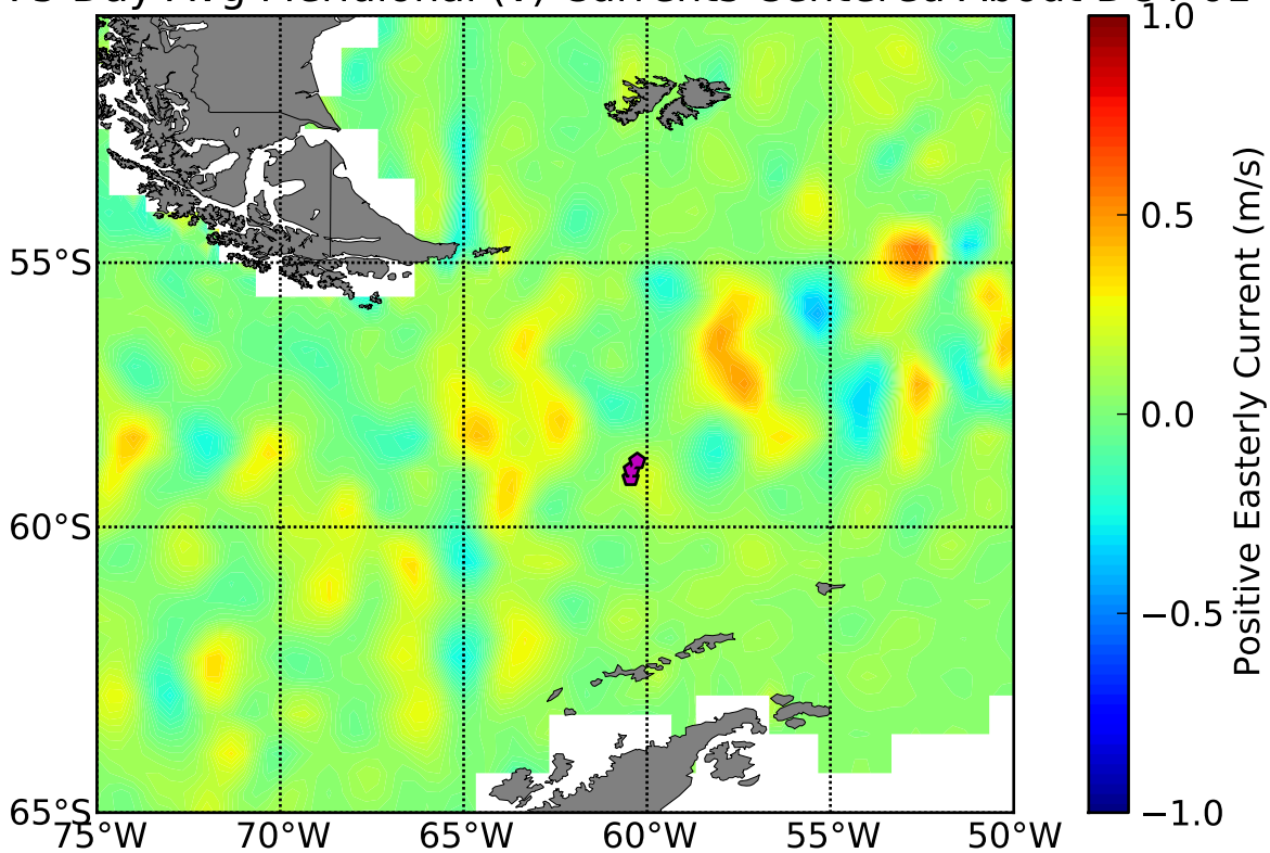
OSCAR 5 Day Avg Meridional (v) Currents Centered About DOY 61
