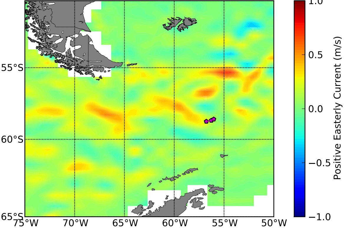
OSCAR 5 Day Avg Zonal (u) Currents Centered About DOY 77
