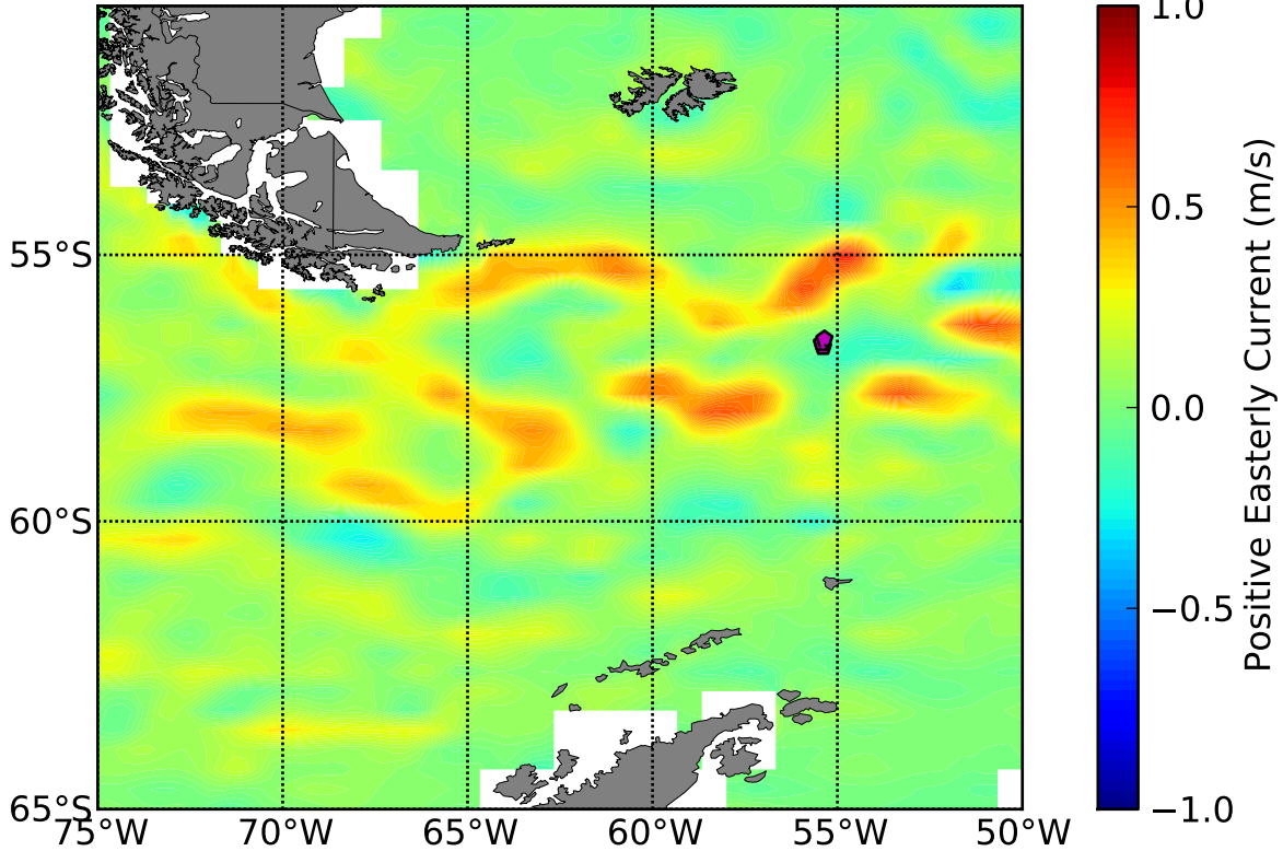
OSCAR 5 Day Avg Zonal (u) Currents Centered About DOY 117
