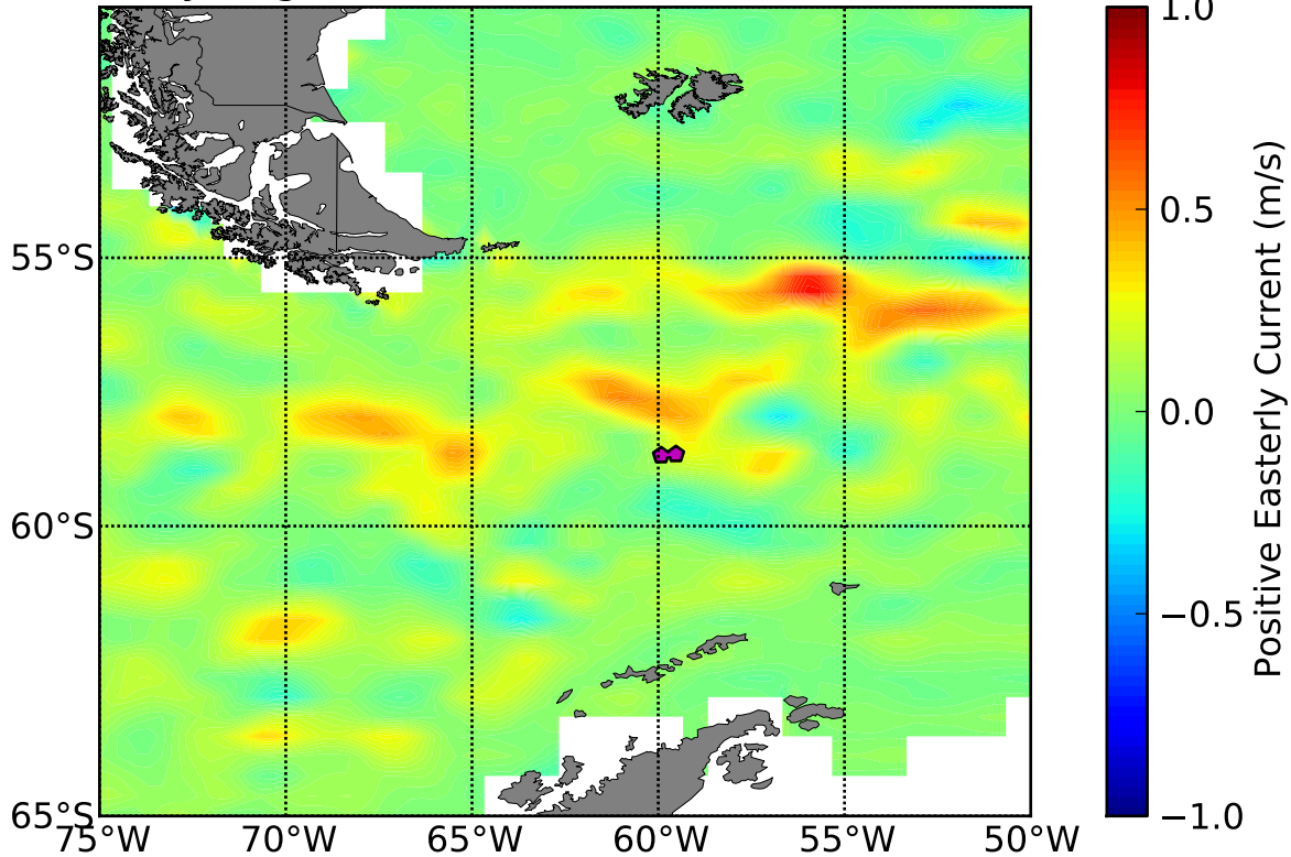
OSCAR 5 Day Avg Zonal (u) Currents Centered About DOY 66
