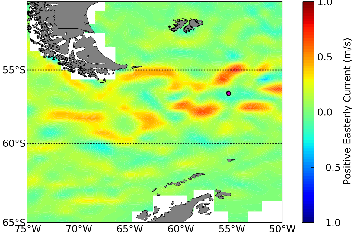
OSCAR 5 Day Avg Zonal (u) Currents Centered About DOY 122
