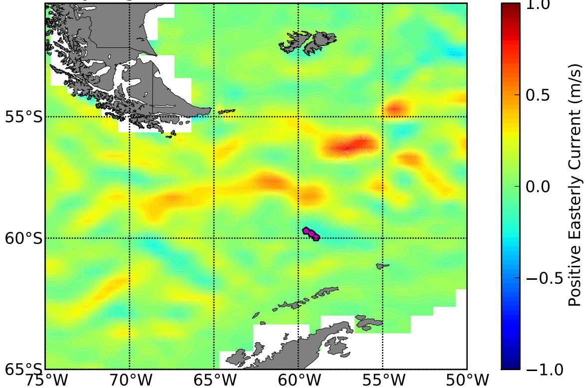
OSCAR 5 Day Avg Zonal (u) Currents Centered About DOY 36
