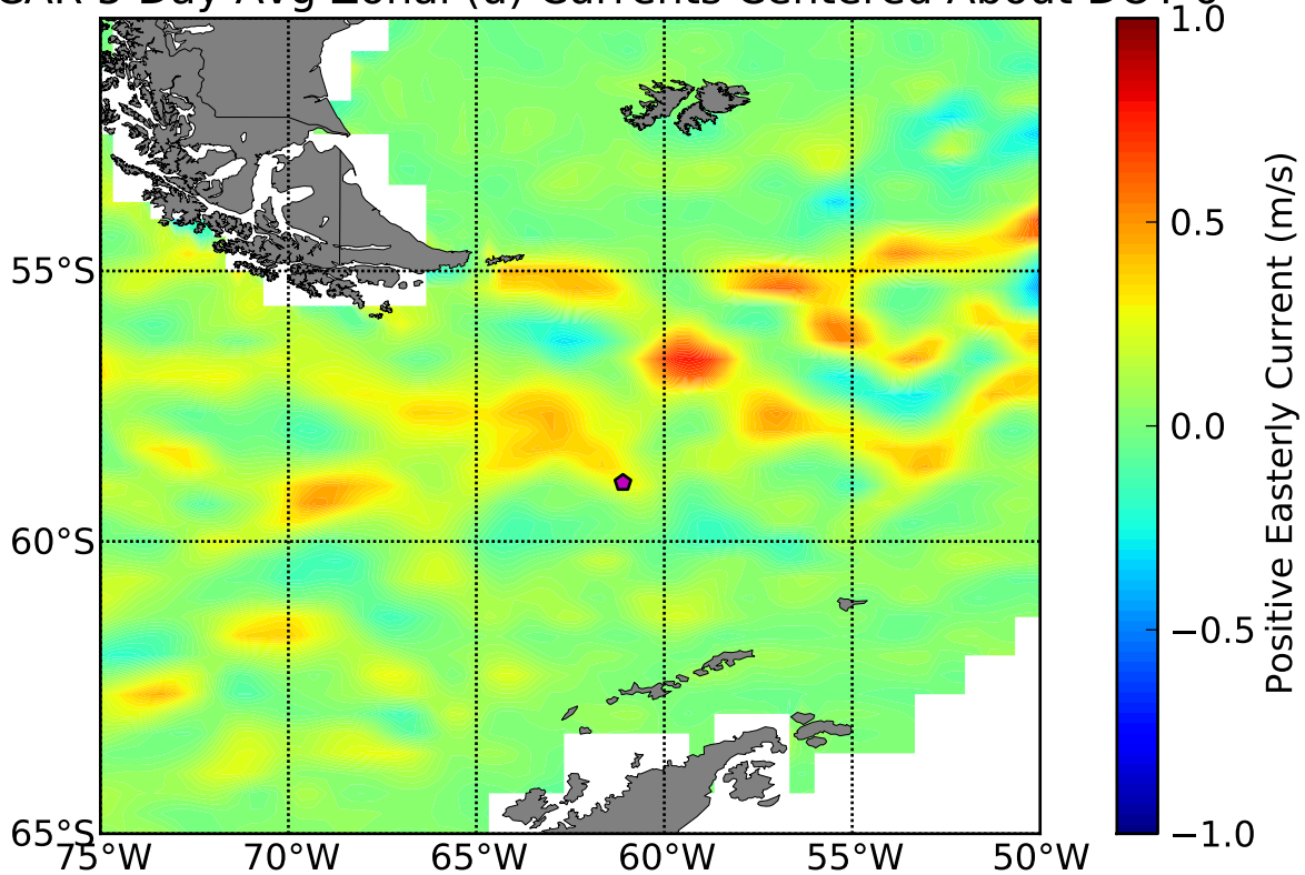
OSCAR 5 Day Avg Zonal (u) Currents Centered About DOY 6
