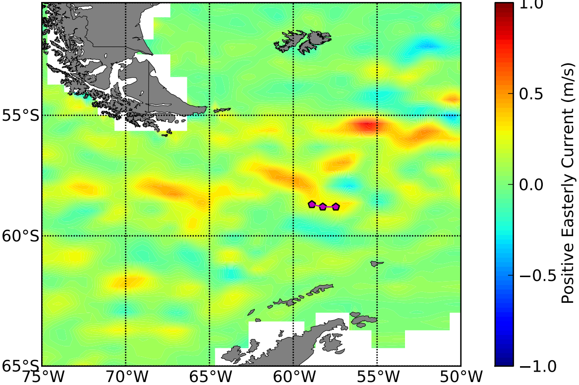
OSCAR 5 Day Avg Zonal (u) Currents Centered About DOY 71
