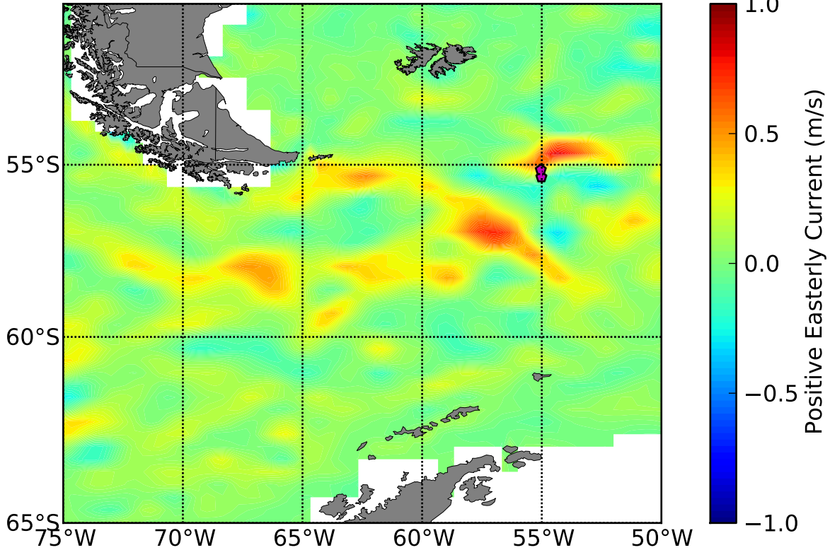
OSCAR 5 Day Avg Zonal (u) Currents Centered About DOY 148
