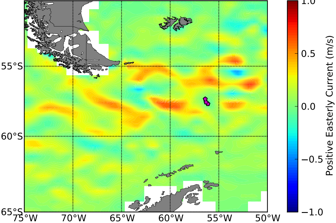
OSCAR 5 Day Avg Zonal (u) Currents Centered About DOY 97
