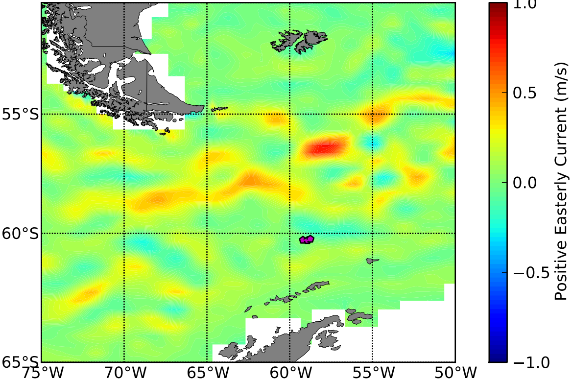
OSCAR 5 Day Avg Zonal (u) Currents Centered About DOY 26
