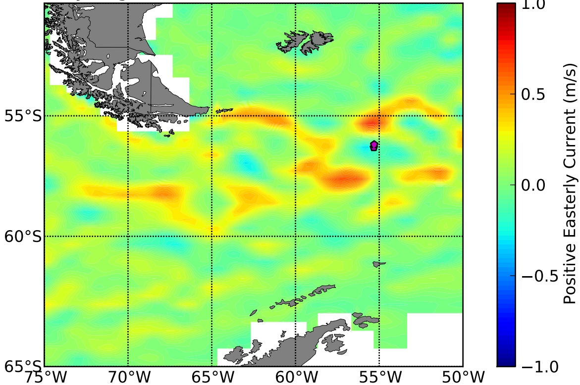
OSCAR 5 Day Avg Zonal (u) Currents Centered About DOY 132
