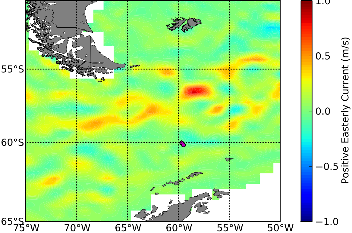
OSCAR 5 Day Avg Zonal (u) Currents Centered About DOY 21
