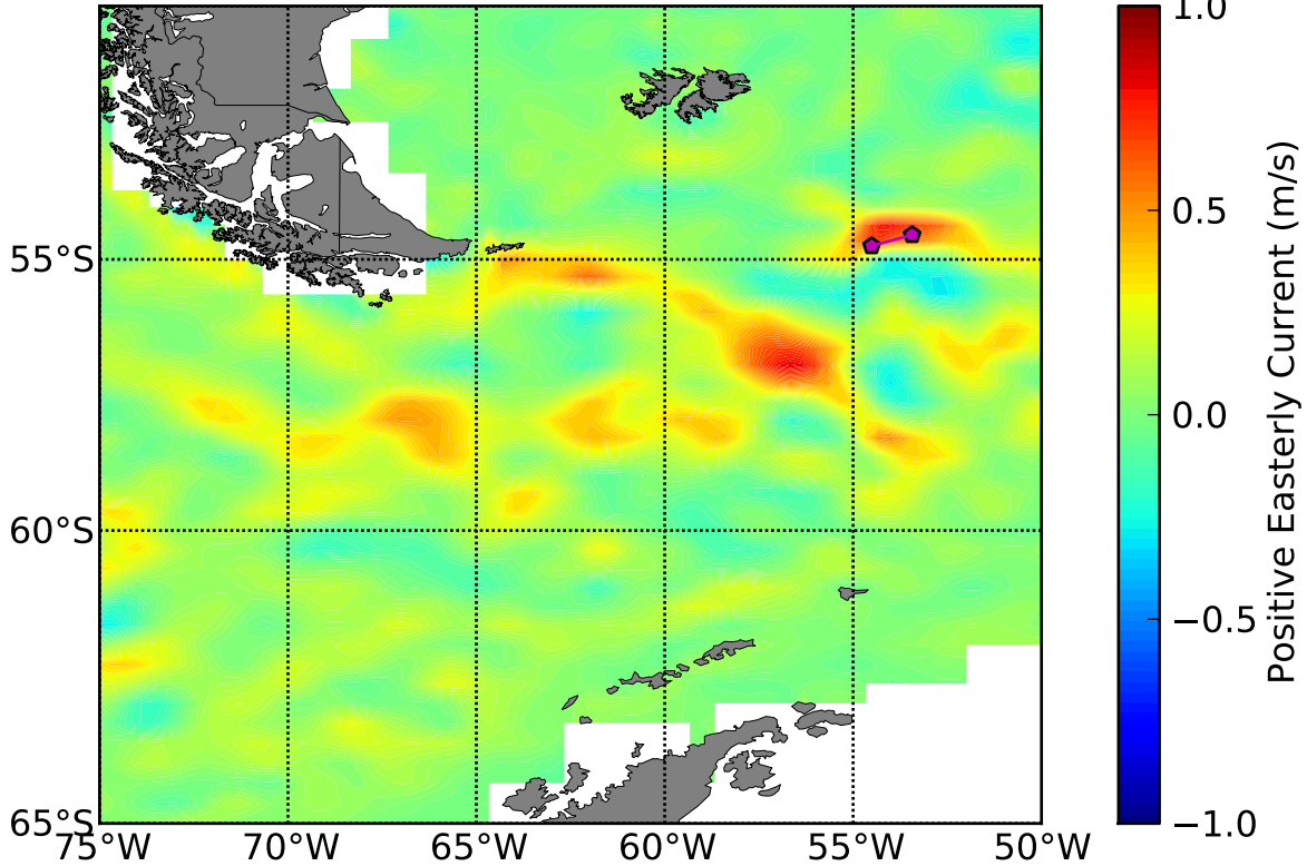
OSCAR 5 Day Avg Zonal (u) Currents Centered About DOY 153
