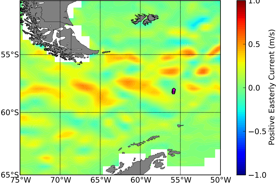
OSCAR 5 Day Avg Zonal (u) Currents Centered About DOY 87
