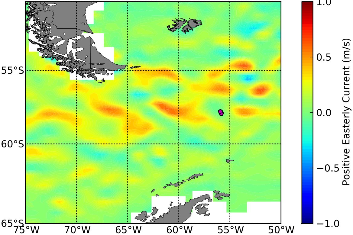
OSCAR 5 Day Avg Zonal (u) Currents Centered About DOY 92
