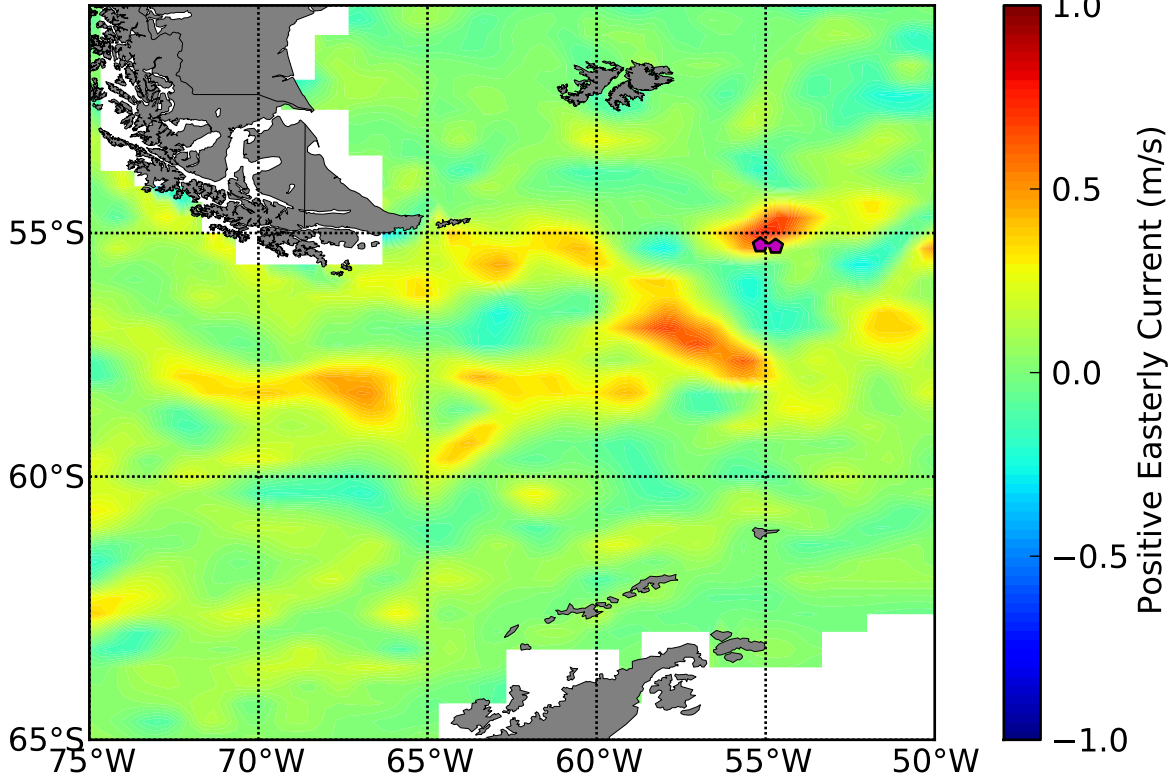
OSCAR 5 Day Avg Zonal (u) Currents Centered About DOY 142
