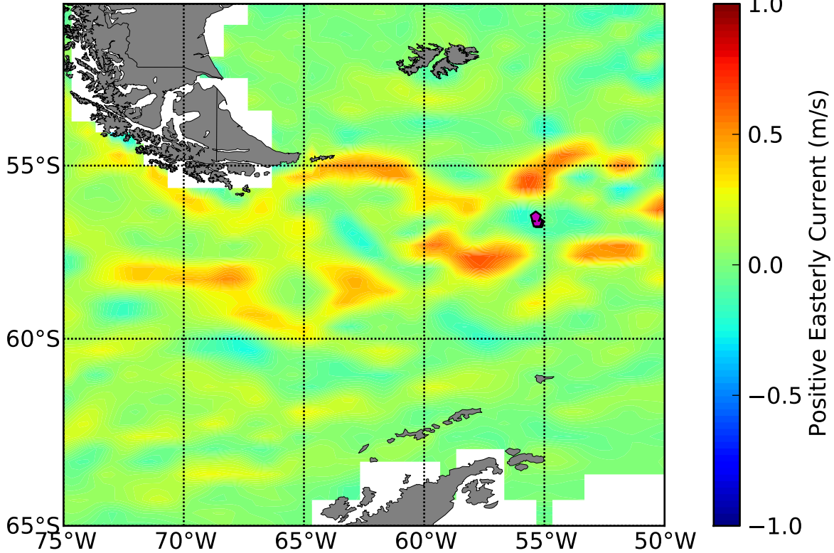
OSCAR 5 Day Avg Zonal (u) Currents Centered About DOY 127
