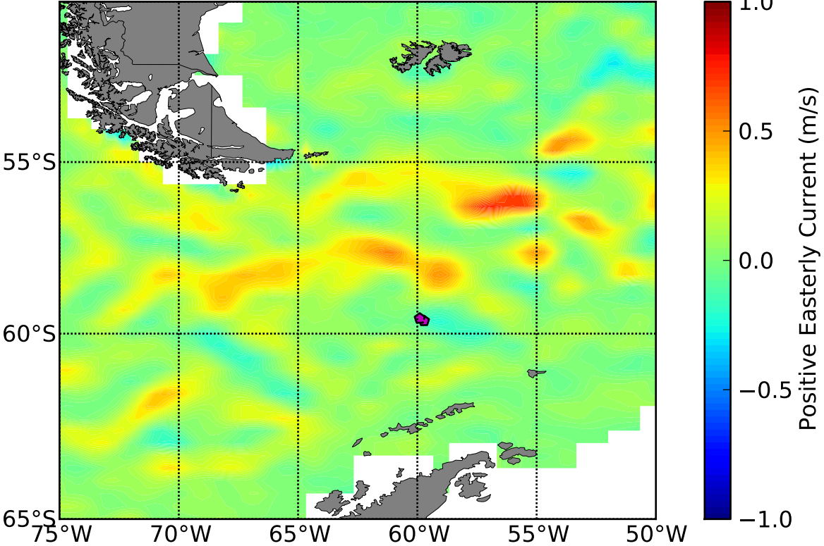
OSCAR 5 Day Avg Zonal (u) Currents Centered About DOY 41
