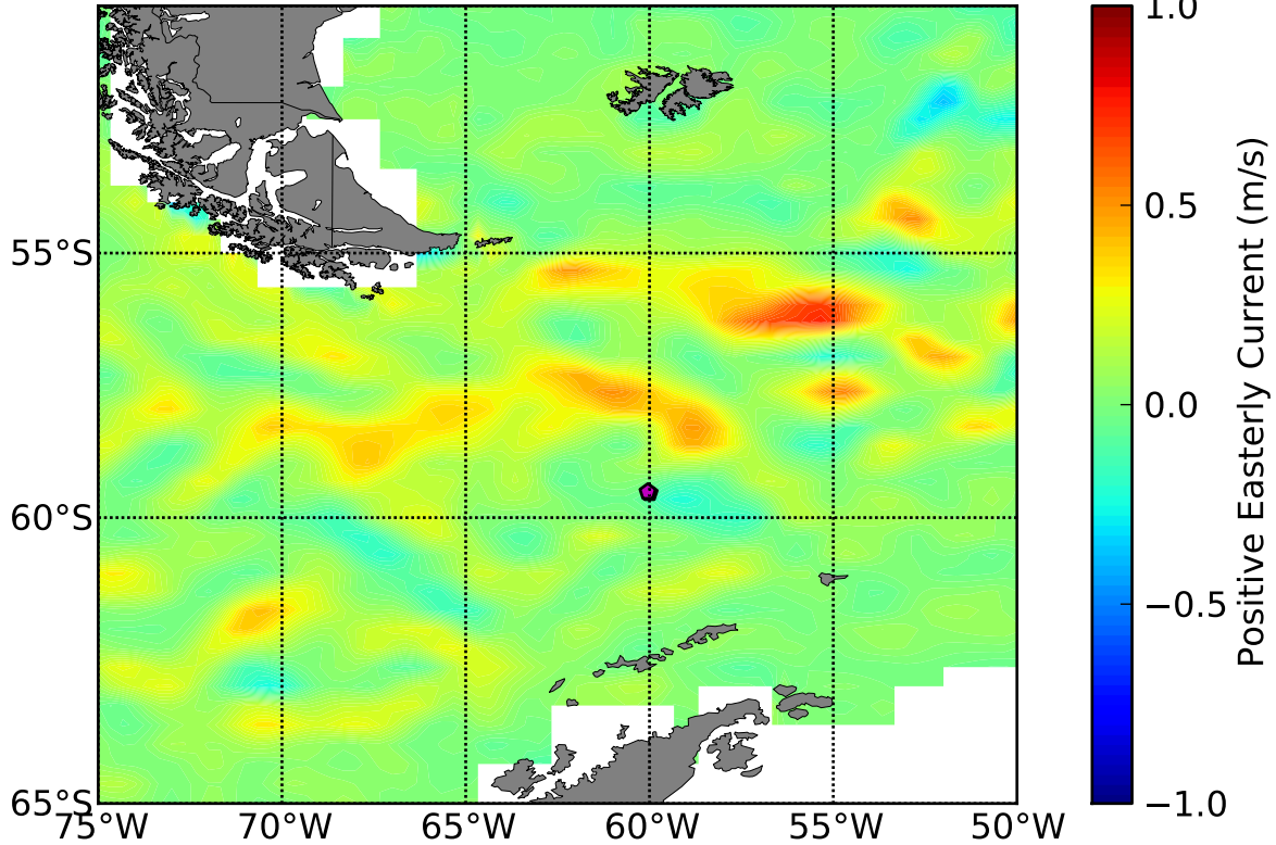
OSCAR 5 Day Avg Zonal (u) Currents Centered About DOY 46
