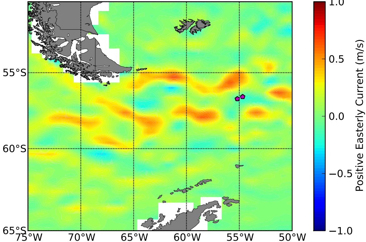
OSCAR 5 Day Avg Zonal (u) Currents Centered About DOY 112
