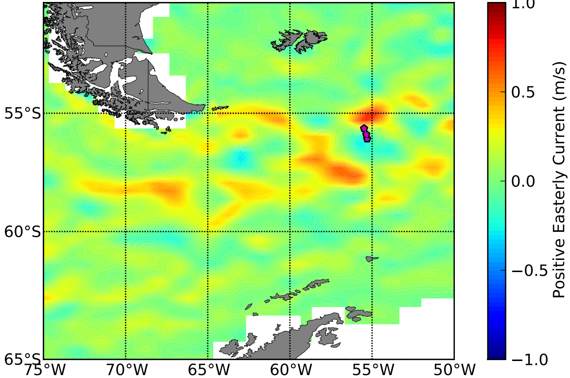
OSCAR 5 Day Avg Zonal (u) Currents Centered About DOY 137
