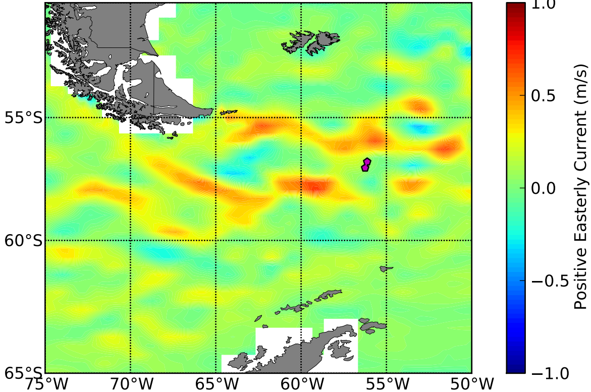
OSCAR 5 Day Avg Zonal (u) Currents Centered About DOY 102
