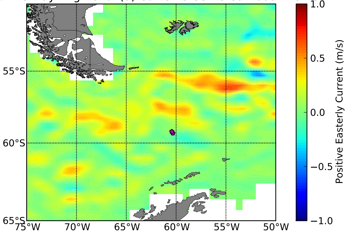
OSCAR 5 Day Avg Zonal (u) Currents Centered About DOY 56
