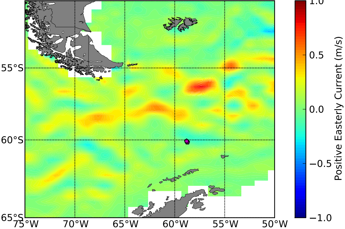
OSCAR 5 Day Avg Zonal (u) Currents Centered About DOY 31
