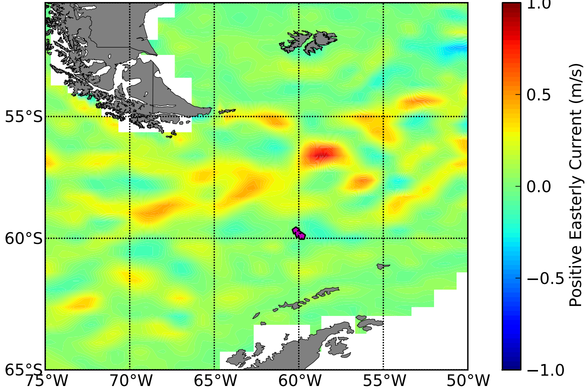
OSCAR 5 Day Avg Zonal (u) Currents Centered About DOY 16
