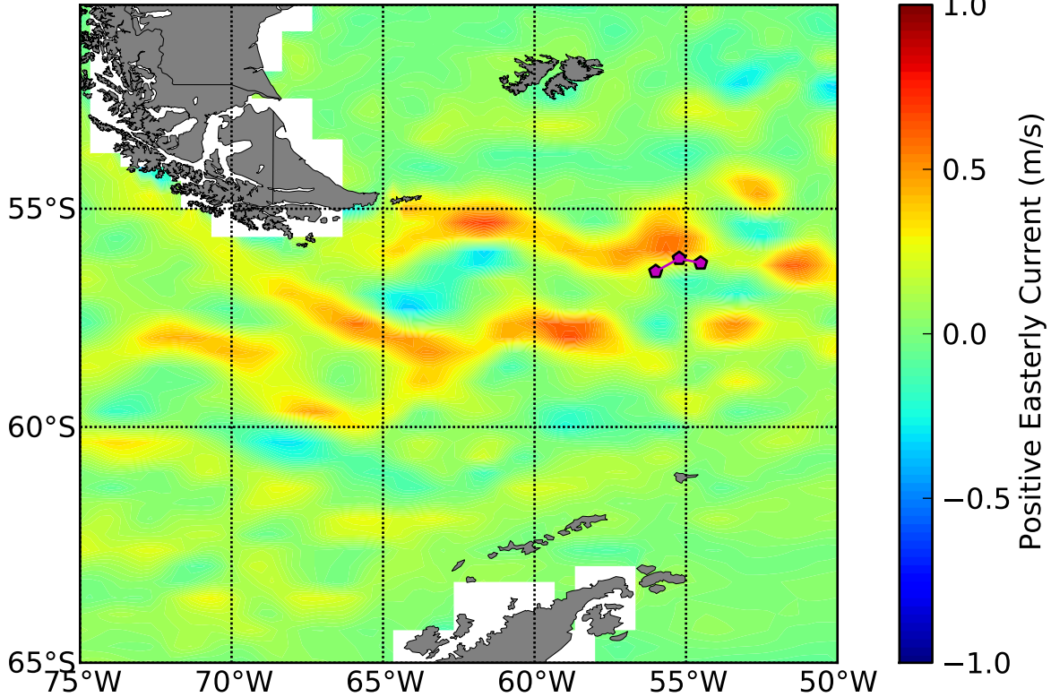
OSCAR 5 Day Avg Zonal (u) Currents Centered About DOY 107
