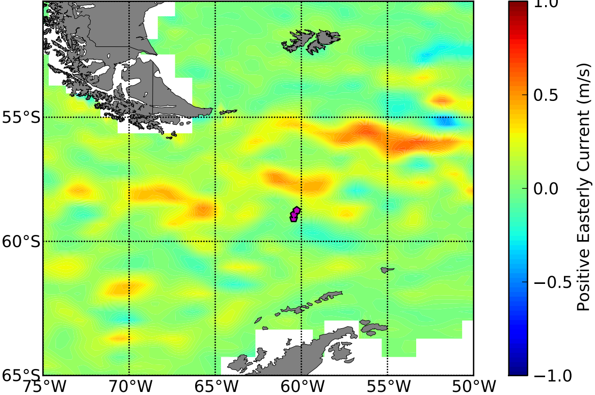
OSCAR 5 Day Avg Zonal (u) Currents Centered About DOY 61
