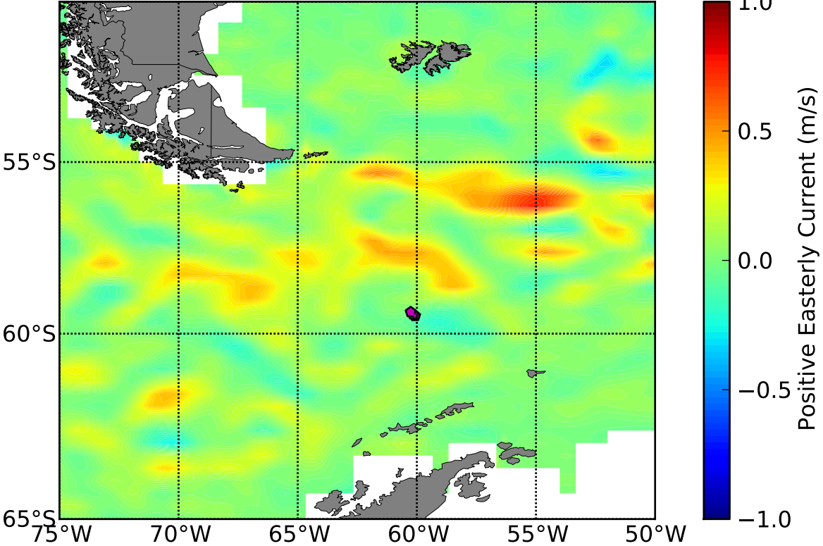
OSCAR 5 Day Avg Zonal (u) Currents Centered About DOY 51
