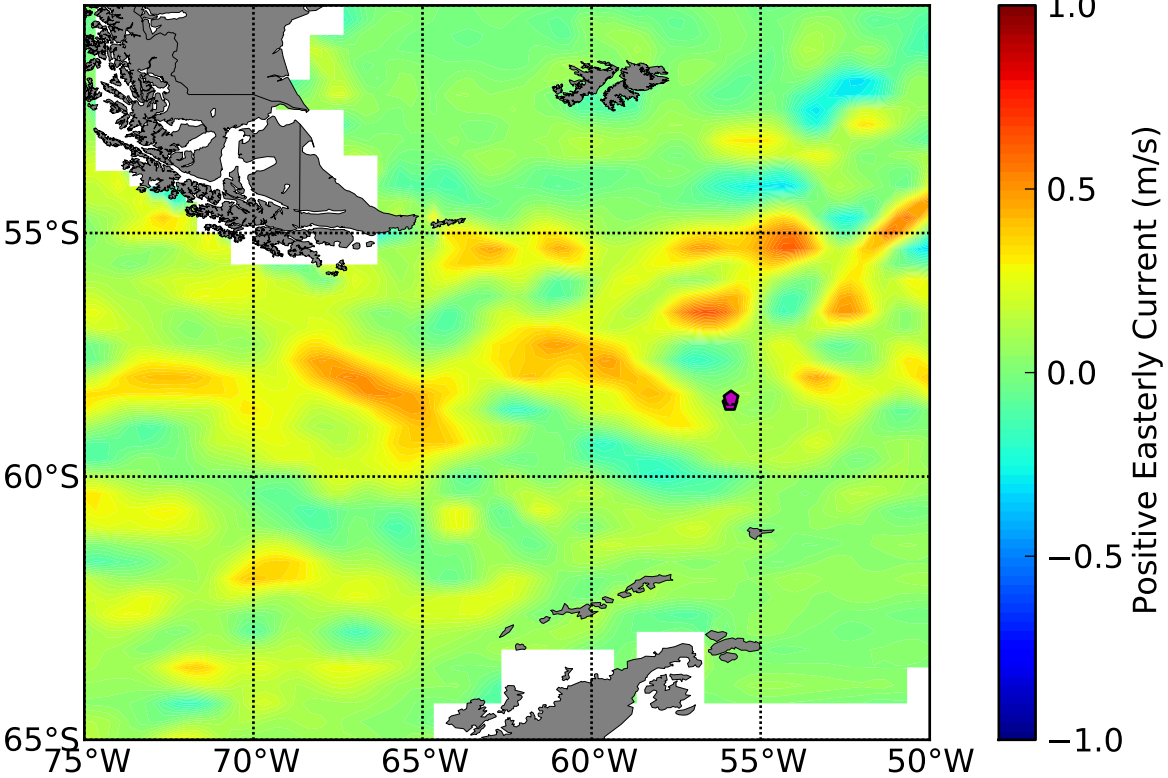
OSCAR 5 Day Avg Zonal (u) Currents Centered About DOY 82
