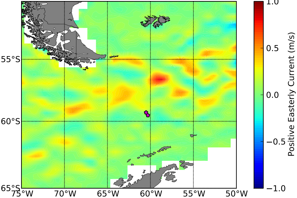
OSCAR 5 Day Avg Zonal (u) Currents Centered About DOY 11
