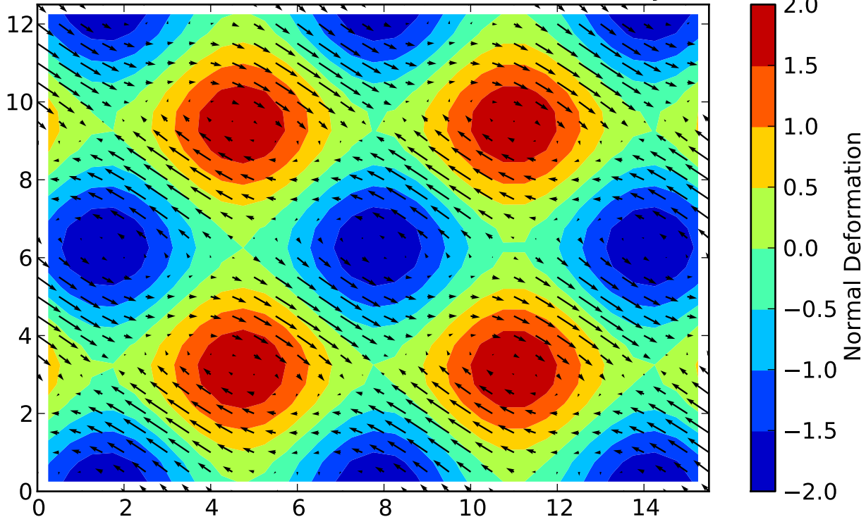
TEST NORMAL DEFORMATION: du/dx-dv/dy
