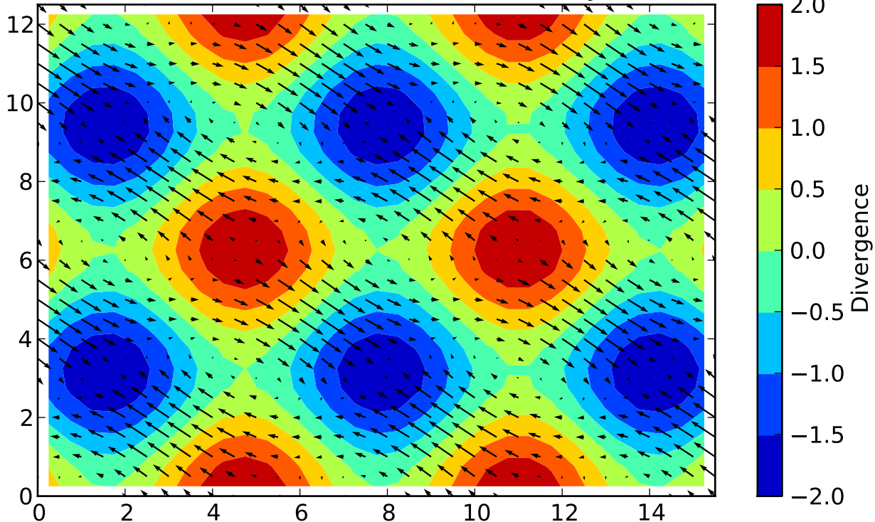
TEST DIVERGENCE: du/dx+dv/dy
