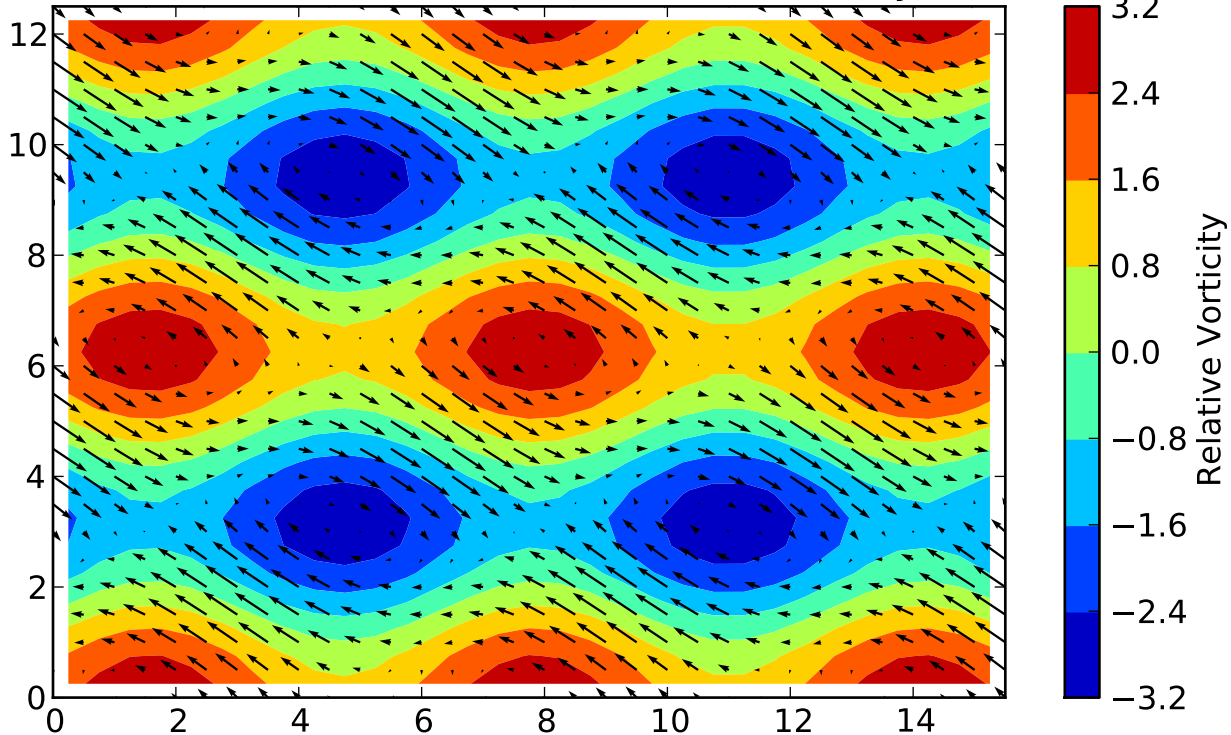
TEST RELATIVE VORTICITY: dv/dx-du/dy
