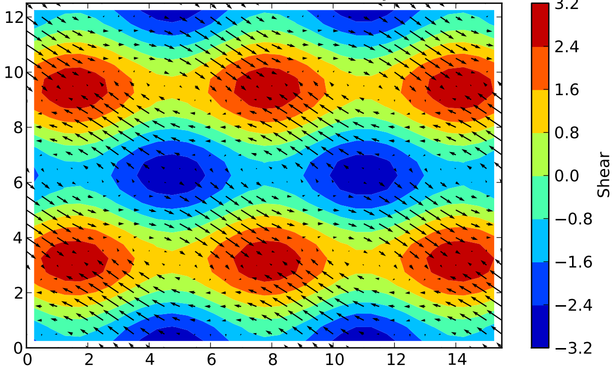
TEST SHEAR: dv/dx+du/dy
