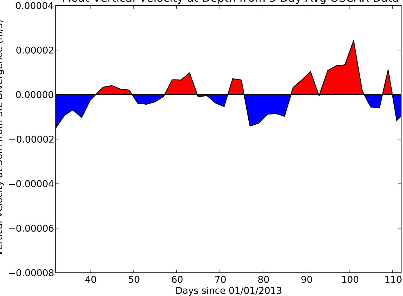
Float Vertical Velocity at Depth from 5 Day Avg OSCAR Data
