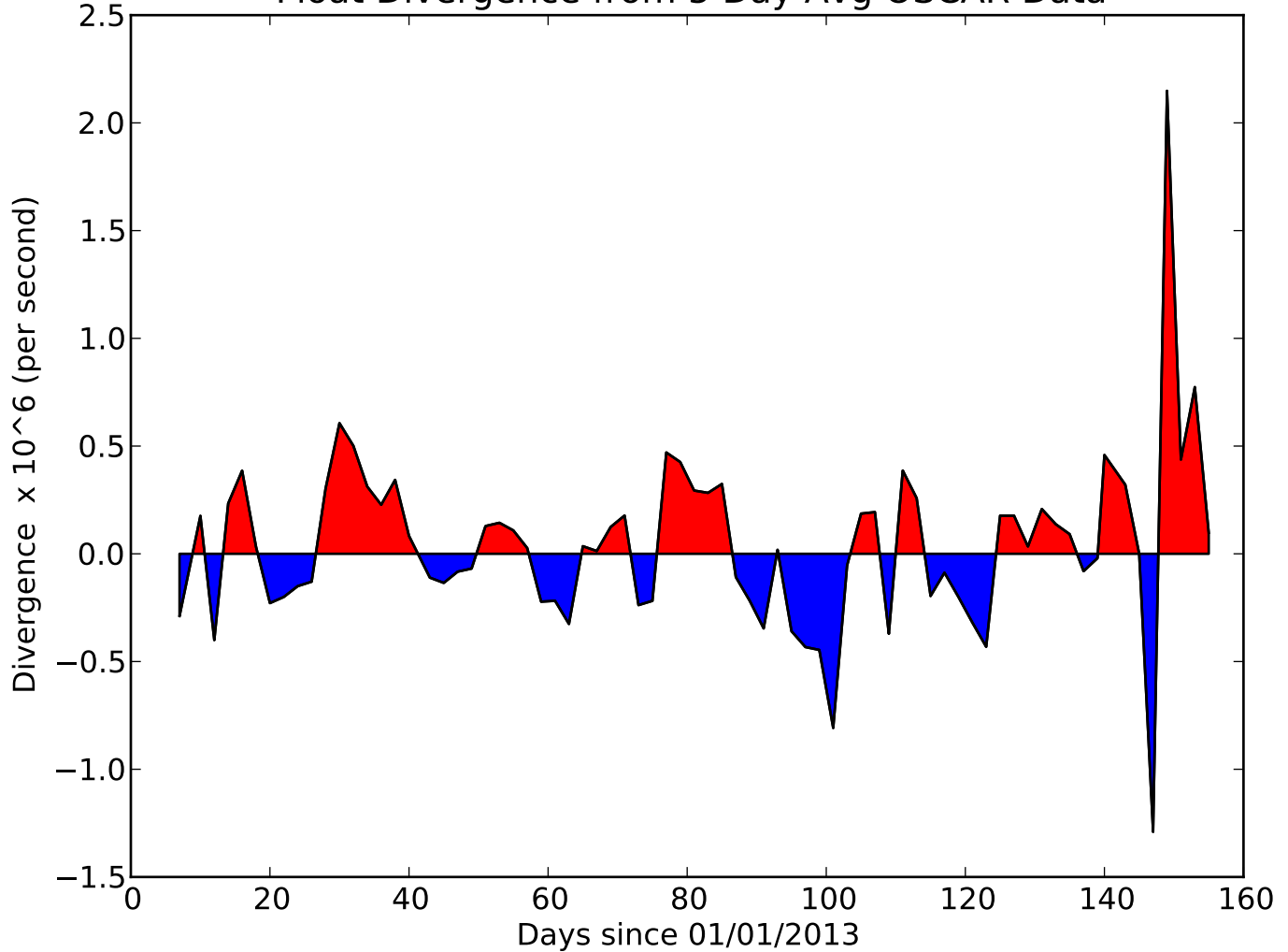
Float Divergence from 5 Day Avg OSCAR Data
