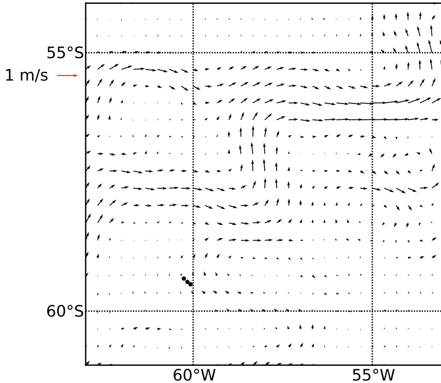
R 5 Day Avg Currents, Float (black), and Tracer (blue) Location Centered About I
