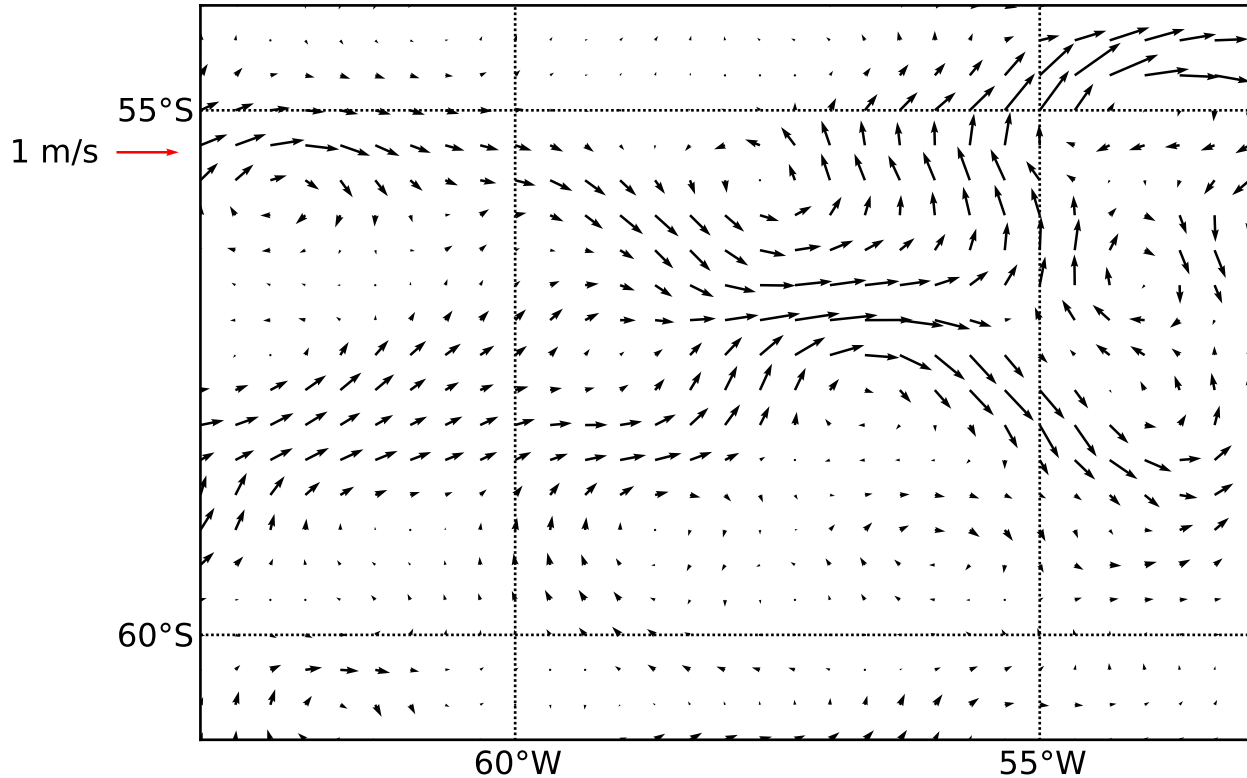
Daily Averaged OSCAR Data on DOY: 150
