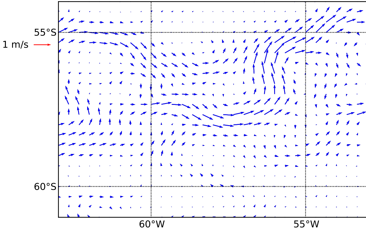
Daily Averaged OSCAR Data on DOY: 127
