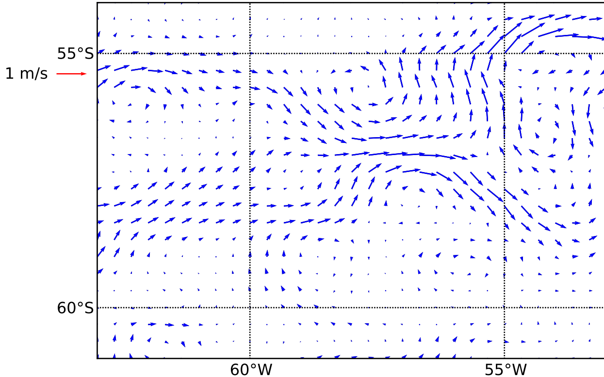
Daily Averaged OSCAR Data on DOY: 148
