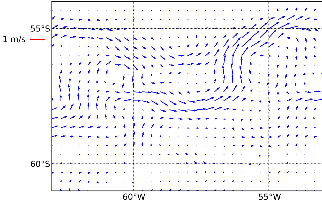
Daily Averaged OSCAR Data on DOY: 122
