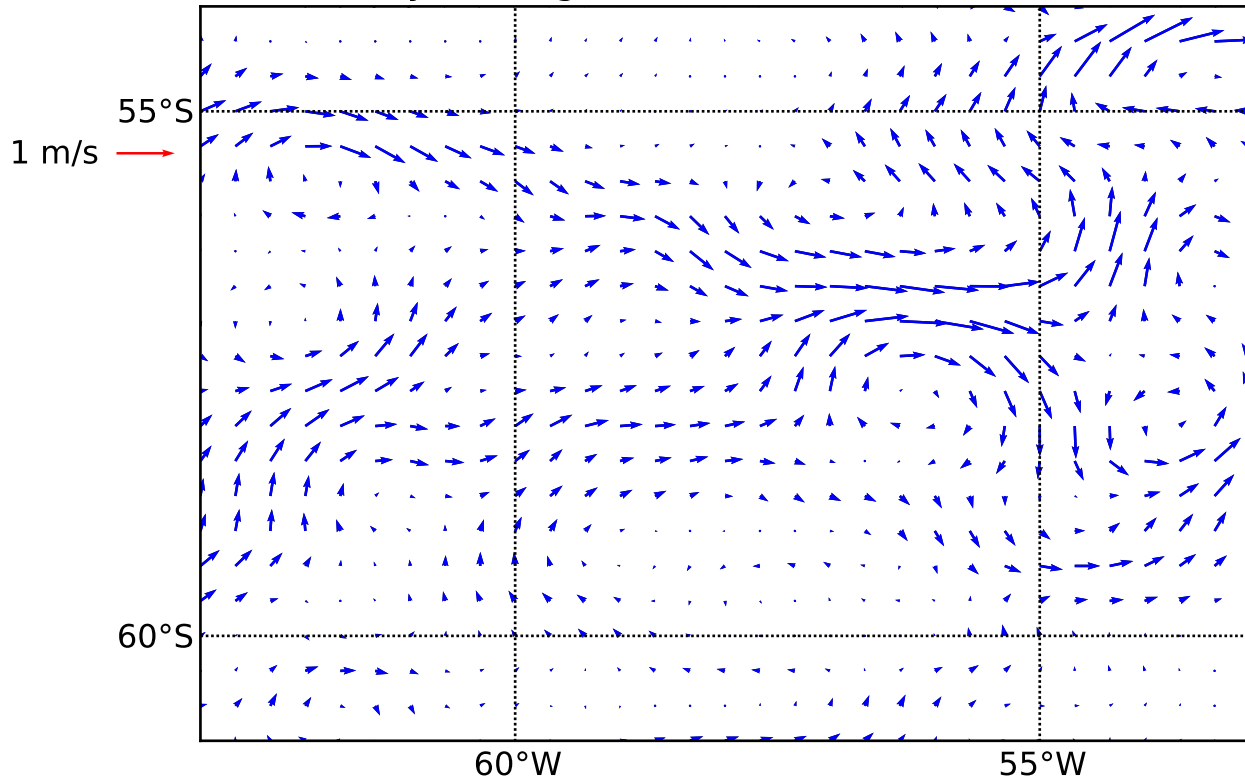
Daily Averaged OSCAR Data on DOY: 158
