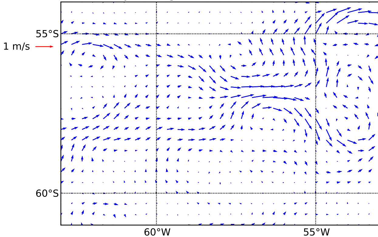
Daily Averaged OSCAR Data on DOY: 153
