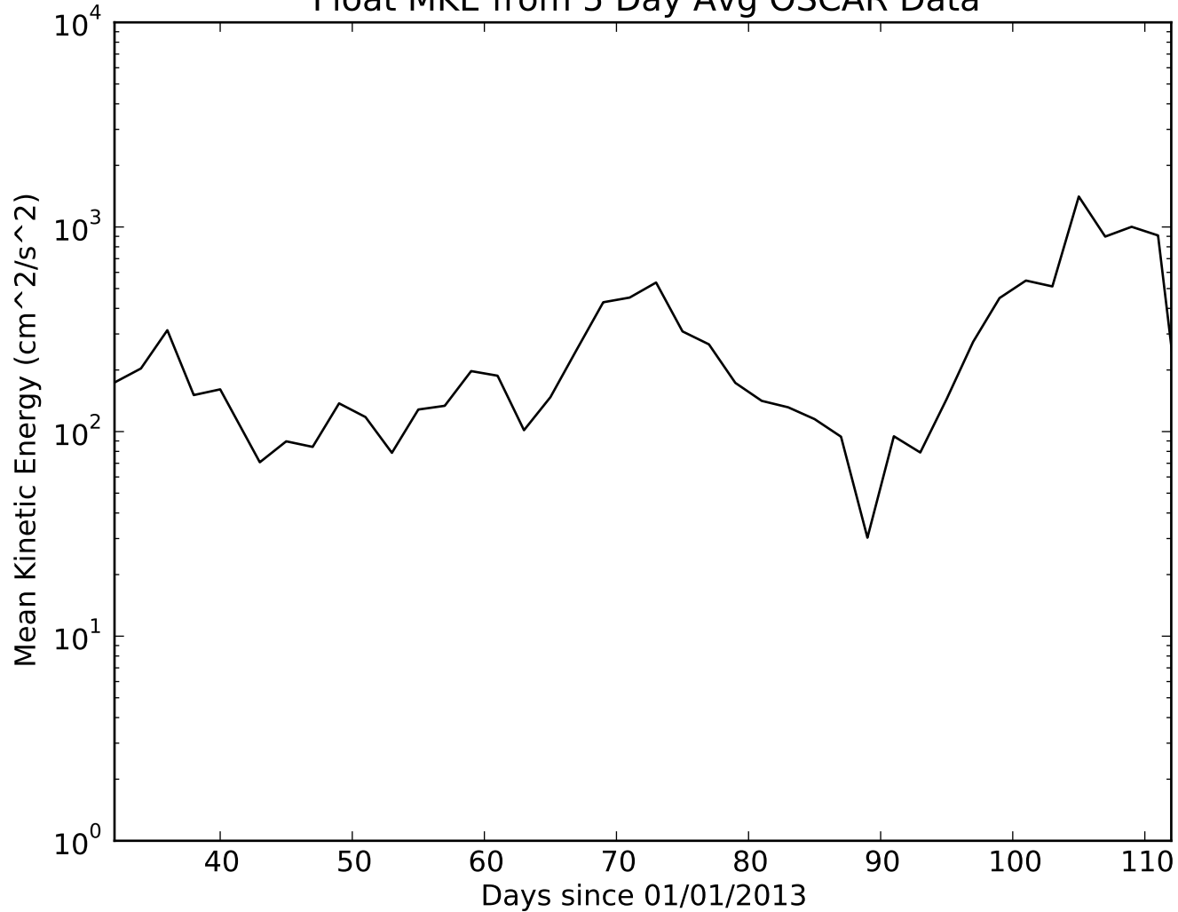
Float MKE from 5 Day Avg OSCAR Data
