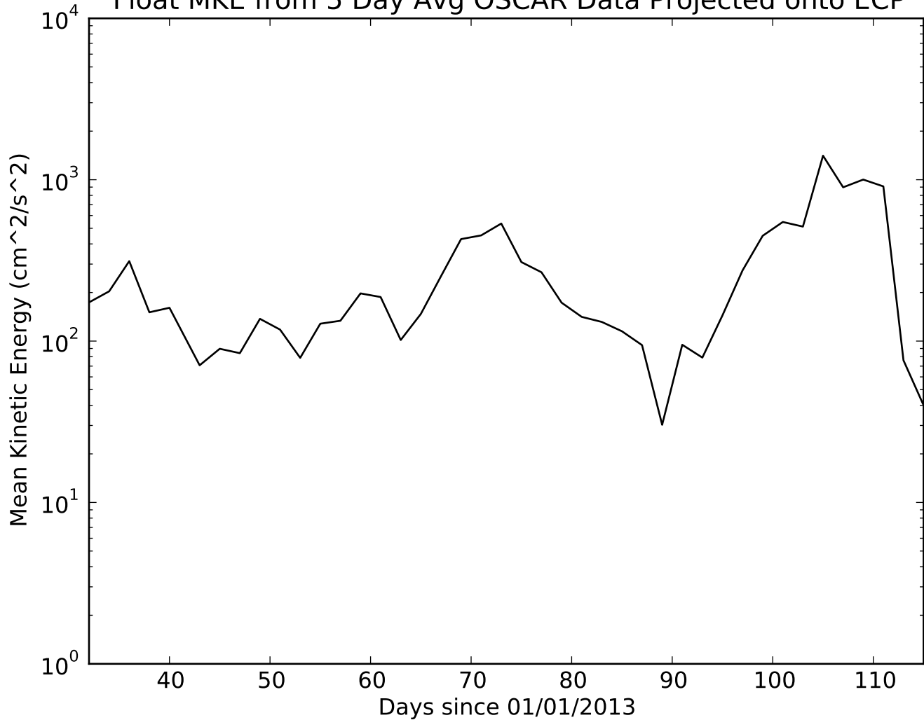
Float MKE from 5 Day Avg OSCAR Data Projected onto ECP
