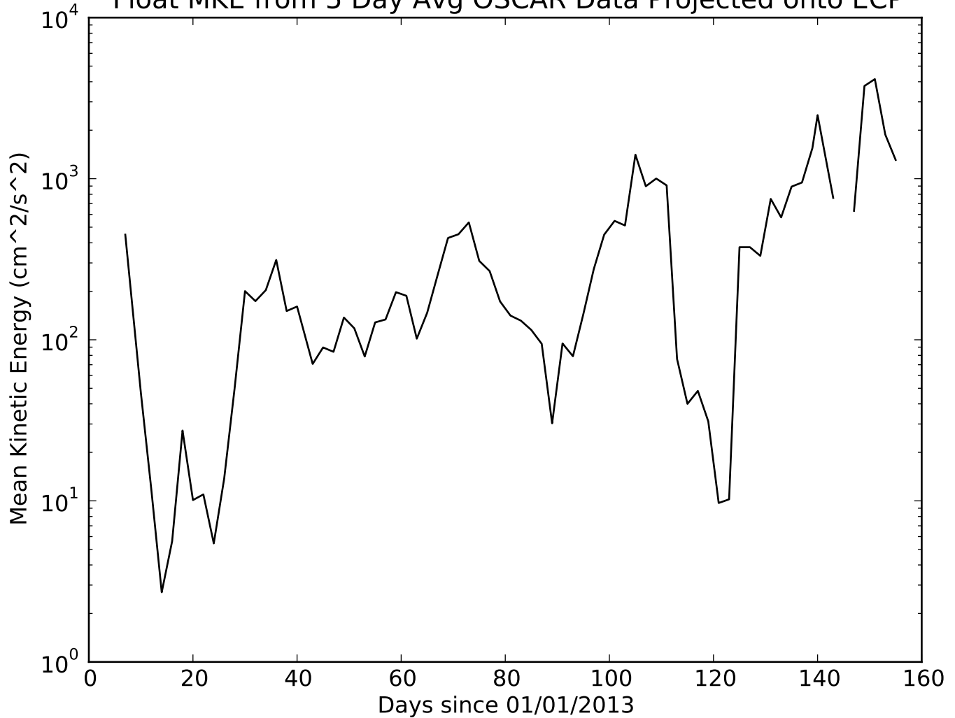
Float MKE from 5 Day Avg OSCAR Data Projected onto ECP
