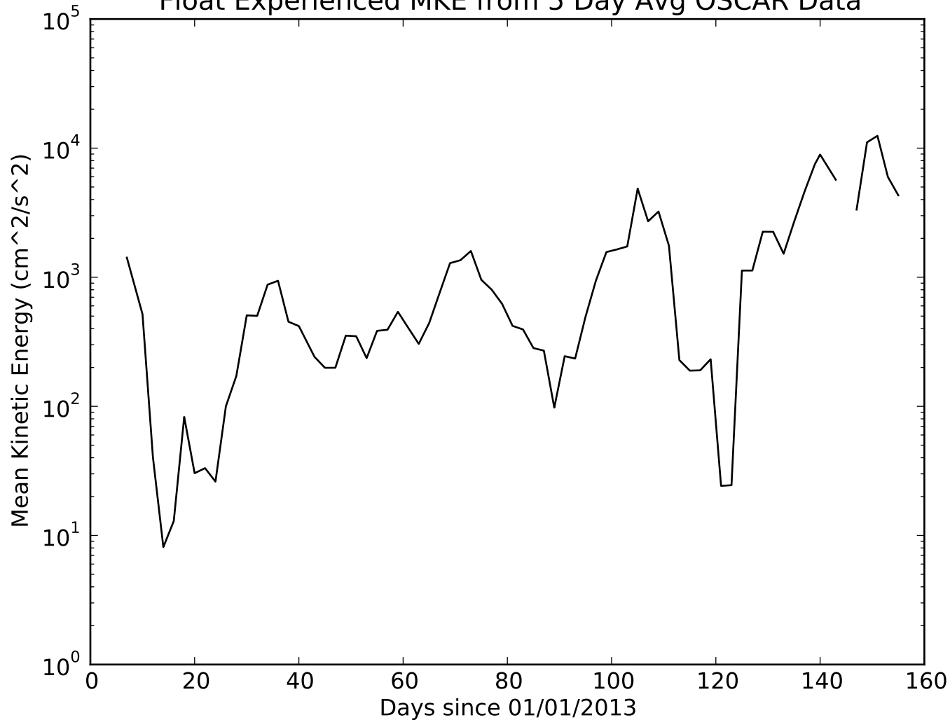
Float Experienced MKE from 5 Day Avg OSCAR Data
